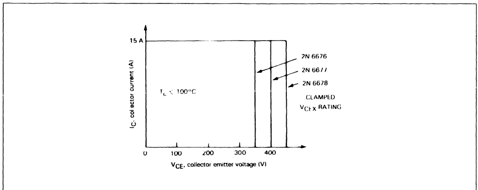
Figure 2 : Maximum Operating Conditions for Switching between Saturation and Cut-off.
