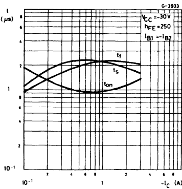
Saturated Switching Characteristics (BDX54S).
