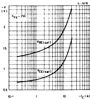
Saturation Voltages (PNP).
