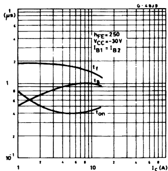
Saturated Switching Characteristics (PNP types).
