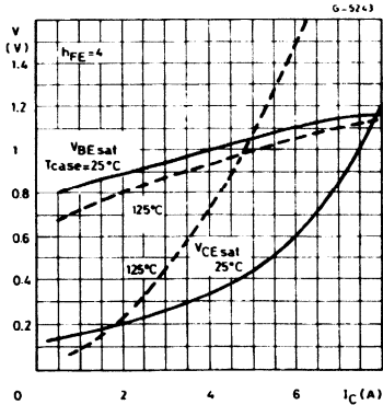
Saturation Voltage.
