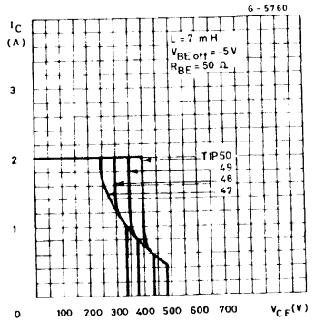
Camped Reverse Bias Safe Operating Areas.
