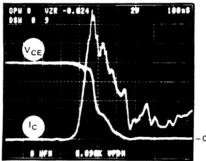
Figure 18: Turn-on for SGSF462.
