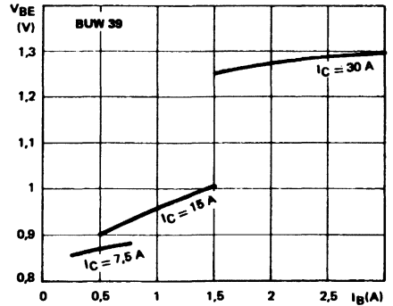
Saturation Voltages.
