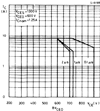
Figure 9: Extension of Safe Operating Area for SGSF425.
