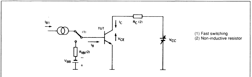
Figure 1 : Switching Times Test Circuit (resistive load).
