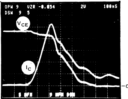
Figure 21: Turn-on for SGSF444. a) Collector Current and Voltage Waveform
