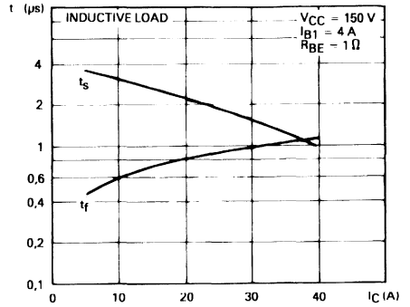
Inductive Load without Negative Base Drive.
