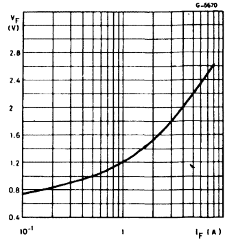
Freewheel Diode Forward Voltage (NPN types).
