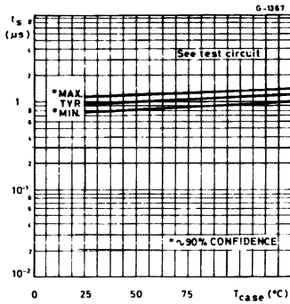
Turn-off Time.
