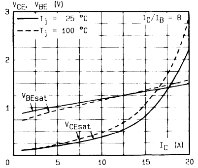
Saturation Voltage.
