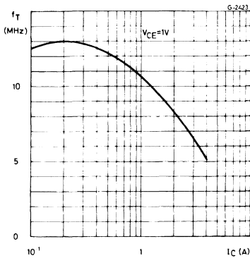
Transition Frequency (NPN type).
