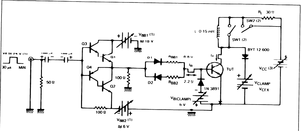
Figure 1 : Switching Time Measurements.
