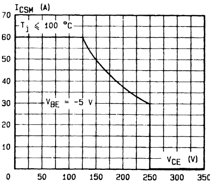
Reverse Biased Accidental Overload Area (RBADA).
