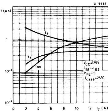
Switching Times Resistive Load (see fig. 2).
