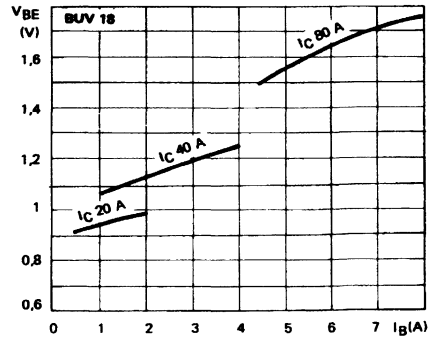
Saturation Voltage.
