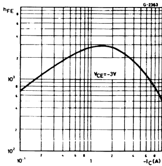
DC Current Gain (PNP types).
