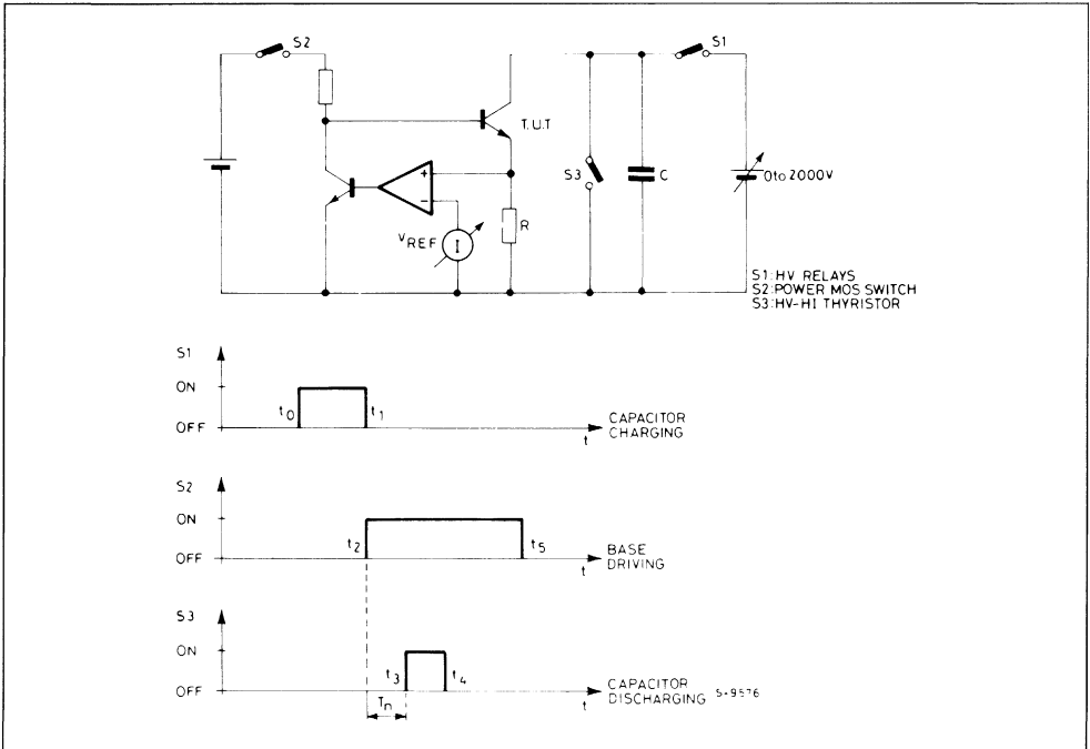
Figure 2: Measurement Circuit.
