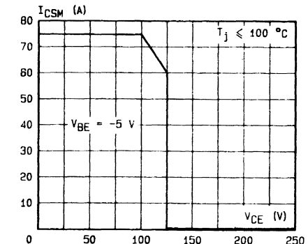
Reverse Biased Accidental Overload Area (RBADA).
