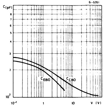
Capacitances (NPN type).
