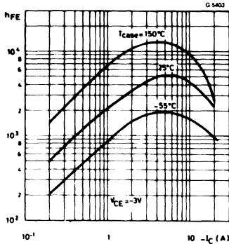
DC Current Gain (PNP types).
