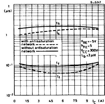
Switching Time Inductive Load (see fig. 2).
