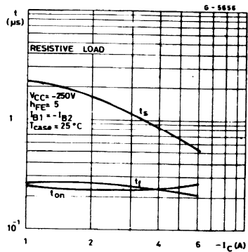
Saturated Switching Characteristics (test circuit fig. 1).
