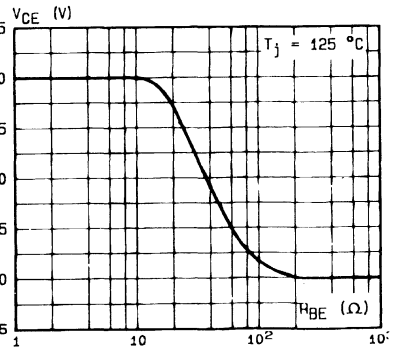
Collector-emitter Voltage vs. Base emitter Resistance.
