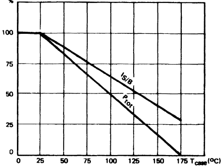
Power and I_{S/B} Derating vs. Case Temperature.
