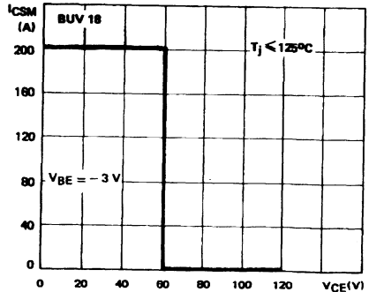
Reverse Biased Accidental Overload Area (RBAOA).
