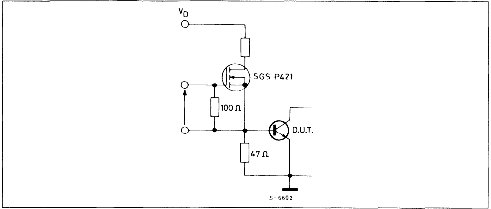
Figure 4 : V_{CE(sat)} Dyn. Test Circuit.
