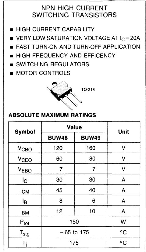
Figure 1 - An extract from the BUW 48 data sheet. The principal characteristics are specified on the upper right hand side.
