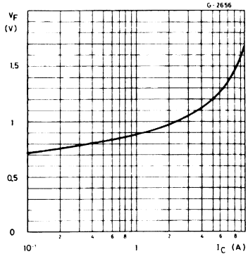
Forward Voltage.
