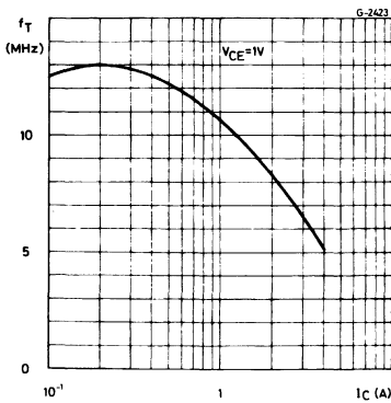
Transition Frequency (NPN types).
