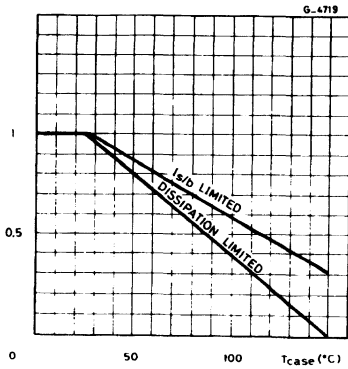
Derating Curves.
