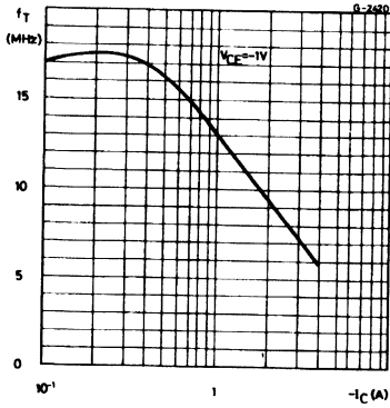
Transition Frequency (PNP types).
