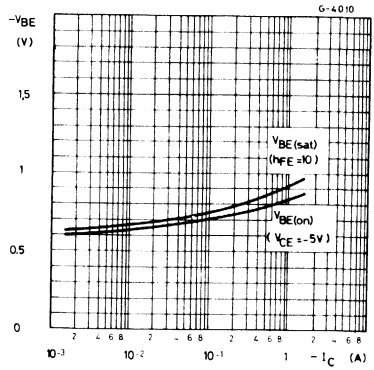
Base-emitter Voltage.
