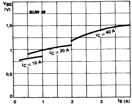
Saturation Voltages.
