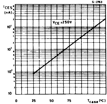
Collector Cutoff Current.
