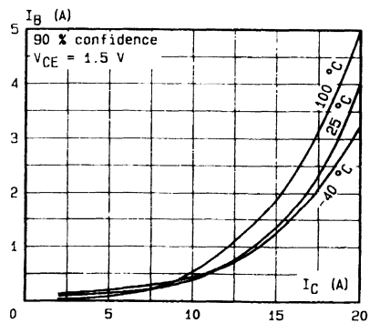
Minimum Base Current to saturate the Transistor.
