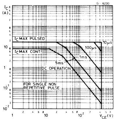
Figure 14: Safe Operating Area for SGSF442.
