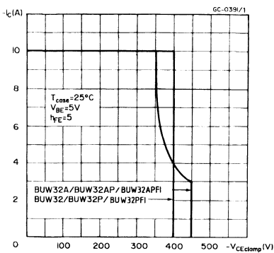
Clamped Reverse Bias Safe Operating Areas.
