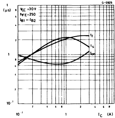
Saturated Switching Characteristics (BDW91)
