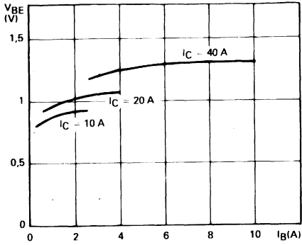
Saturation Voltage Low Gain.
