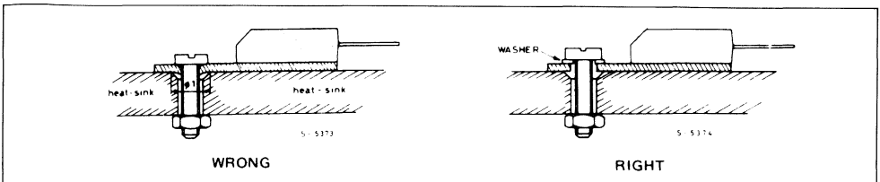
Figure 7 - Device Mounting
