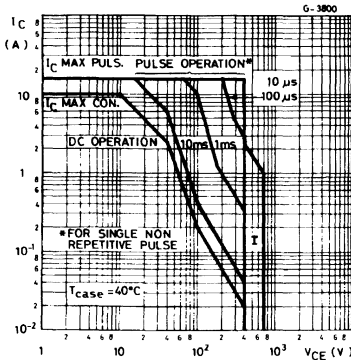
I - Area of permissible operation during Turn-on provided R_{BE} \leq 100\ \Omega and t_b \leq 0.6\ \mu\text{s} .
