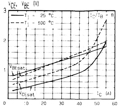
Saturation Voltage.
