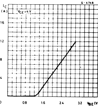
DC Transconductance (TIP145/6/7).
