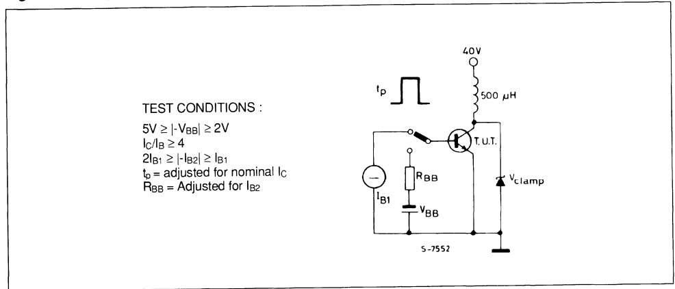
Figure 1 : Clamped Es/b Test Circuit.
