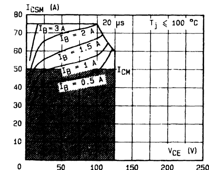
Forward Biased Accidental Overload Area (FBADA).
