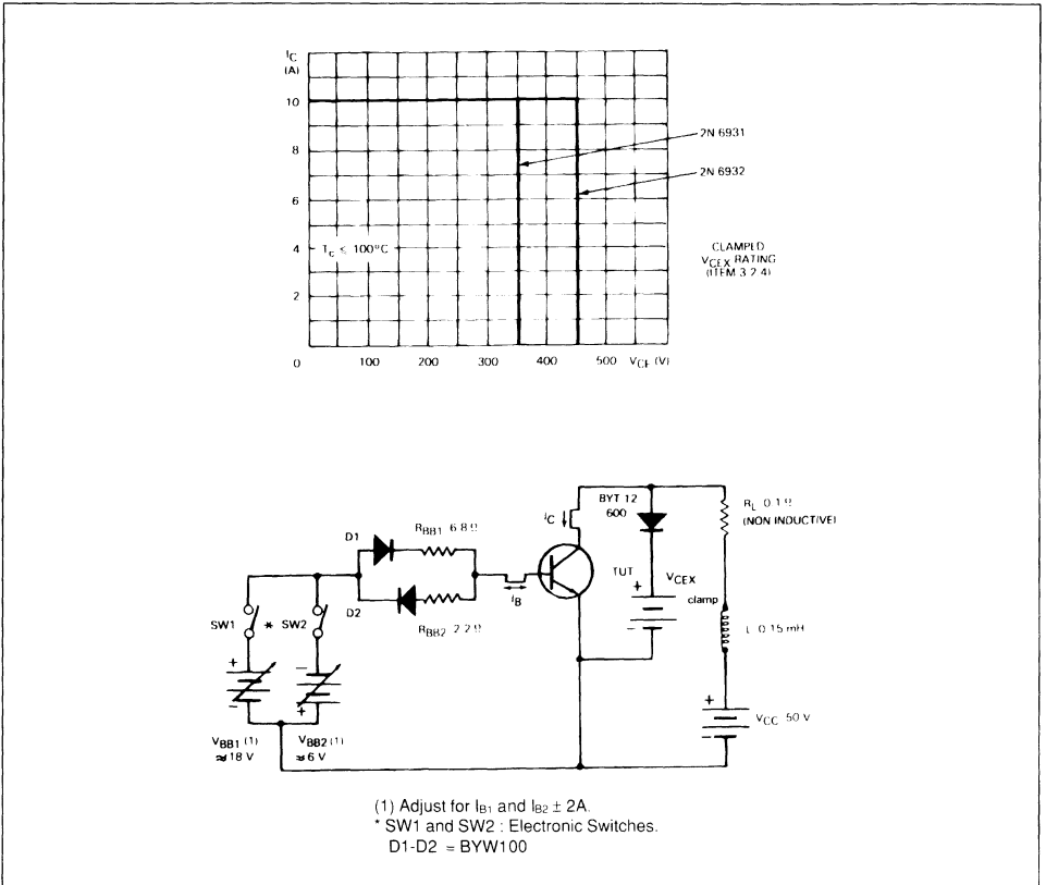
Figure 3 : Maximum Operating Conditions for Switching between Saturation and Cut off.
