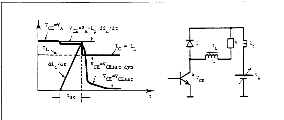
Figure 8 - The turn-on of a transistor with a conducting free-wheeling diode. The transistor constraints are different in comparison to the resistive load case. The voltage V_{CE} remains high during the time t_{sc} .
