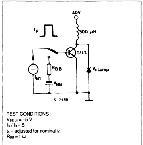
Clamped E_{sb} Test Circuit.
