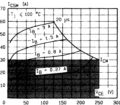
Forward Biased Accidental Overload Area (FBADA).
