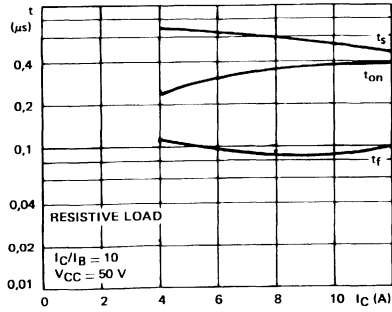
Switching Times vs. Collector Current (resistive load).
