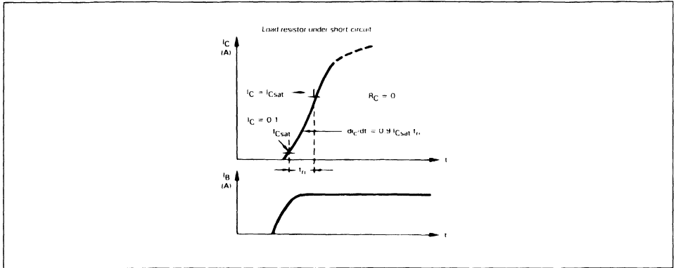
Figure 3 : Maximum Operating Conditions for Switching between Saturation and Cut off.
