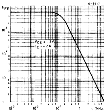
Small Signal Current Gain (PNP types).
