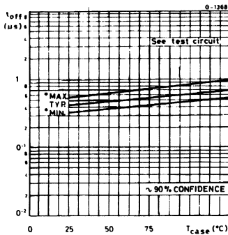
Turn-off Time.
