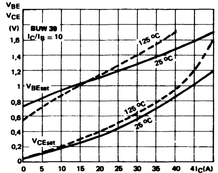
Saturation Voltages.
