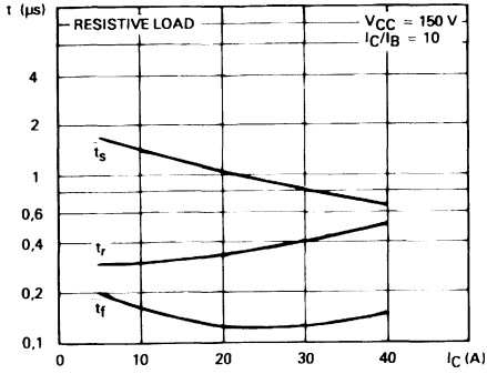
Switching Times vs. Collector Current (resistive load).
