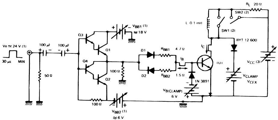
Figure 1 : Switching Time Measurements.
