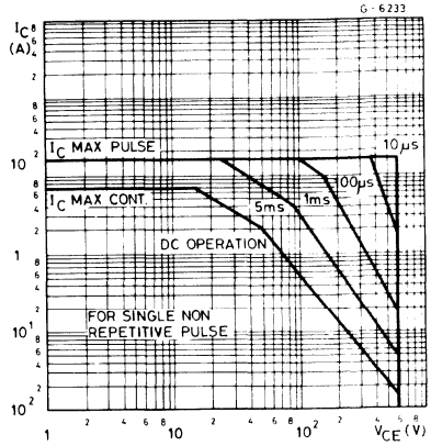
Figure 20: Safe Operating Area for SGSF444.
