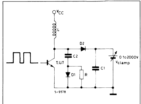
Figure 4: Application Circuit.
