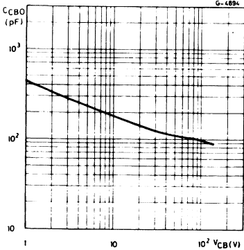
Collector-base Capacitance.
