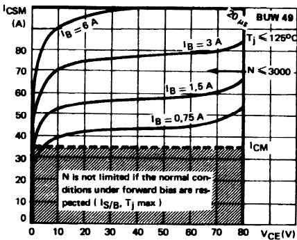
Figure 25 : Forward Biased Accidental Overload Area (FBAOA).
