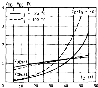
Saturation Voltage.
