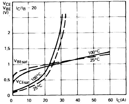
Saturation Voltage High Gain.
