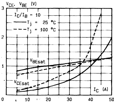
Saturation Voltage.
