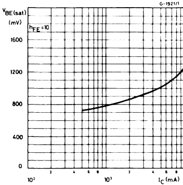
Base-emitter Saturation Voltage.
