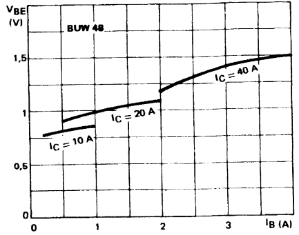
Saturation Voltage.
