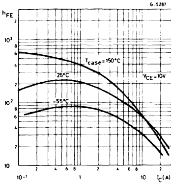
DC Current Gain (PNP types).
