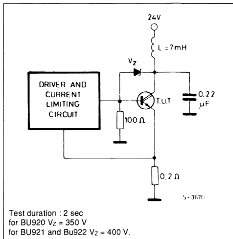
Figure 2 : Functional Test Circuit.
