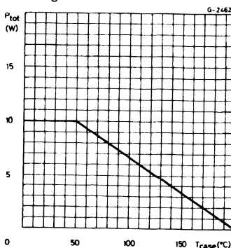
Power Rating Chart.
