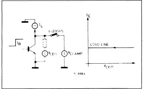
Figure 7: Blocked Diode.
